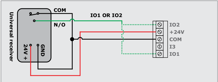
FIGURE 84. WIRING A UNIVERSAL RECEIVER TO THE SDO5 SMART+
