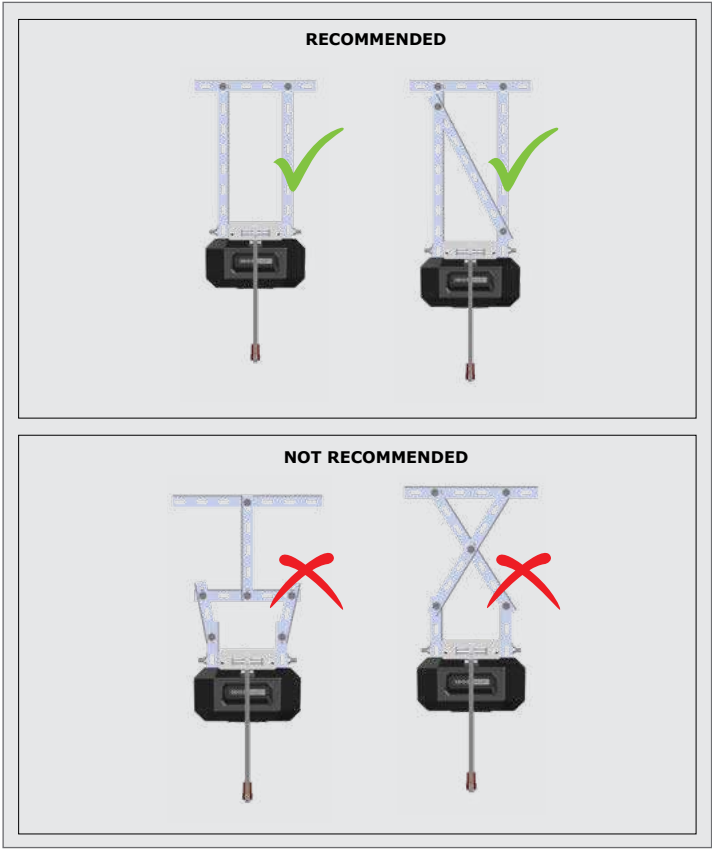
FIGURE 31. CORRECT AND INCORRECT MOUNTING CONFIGURATIONS
