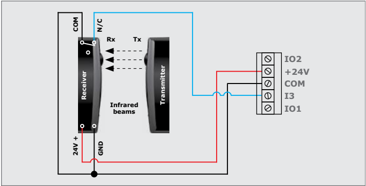
FIGURE 82. WIRING PHOTON SAFETY BEAMS TO THE SDO5 SMART+ (FOUR-WIRE)
