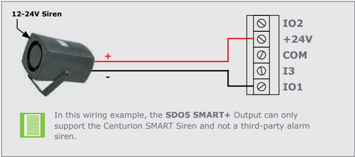
FIGURE 86. SMART SIREN CONNECTED TO SDO5 SMART+
