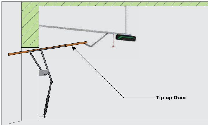
FIGURE 6. TIP UP DOORS
