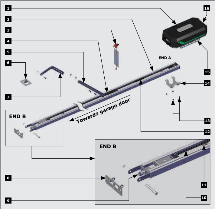
FIGURE 2. SDO5 SMART+ PRODUCT IDENTIFICATION
