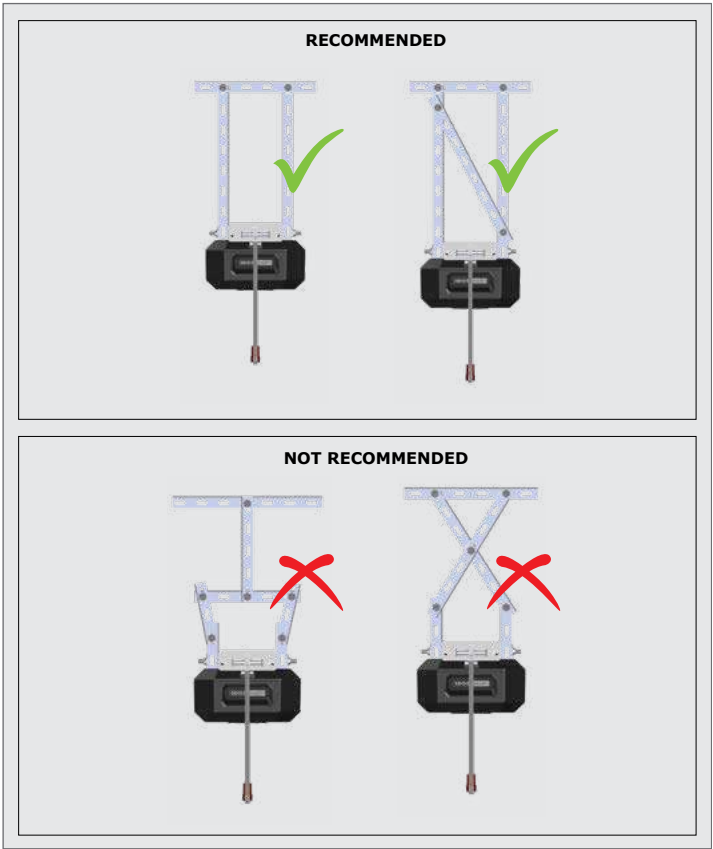
FIGURE 63. CORRECT AND INCORRECT MOUNTING CONFIGURATIONS
