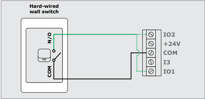
FIGURE 85. HARD-WIRING A WALL SWITCH TO THE SDO5 SMART+
