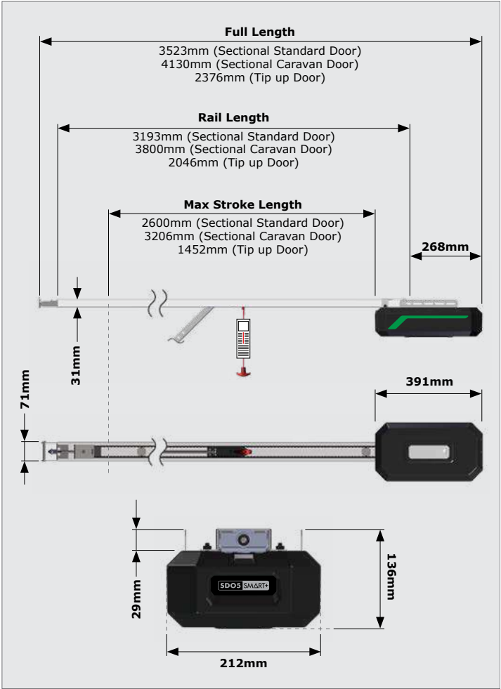
FIGURE 1. OVERALL DIMENSIONS FOR THE SD05 SMART+
